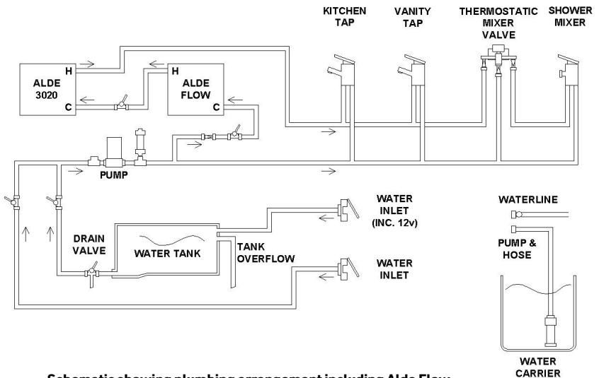
Schematic showing plumbing arrangement including Alde Flow
